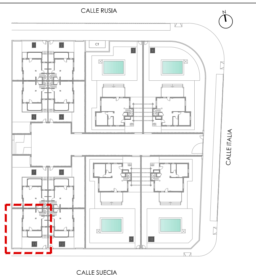
MANZANA 1:650
